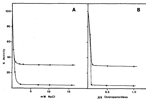
FIGURE 2. Chloride and Enzyme Dependence of Inactivation.
