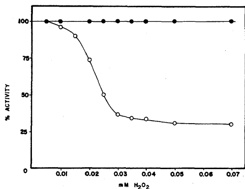
FIGURE 1. Inactivation of B. subtilis \alpha -amylase by chloroperoxidase and variable concentration of H_2O_2 . The incubation mixture contained 10 mM sodium acetate buffer pH 4.8, 60 mM NaCl (1.2 \mu g chloroperoxidase (288 units)) and 1.0 mg of B. subtilis \alpha -amylase in 1.0 ml of solution. Amylase activity was determined by the "Azure Amylase" method (6). ●—● controls (no chloride); ○—○ complete system.
